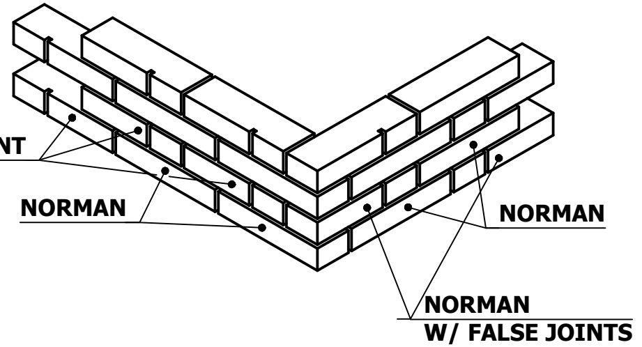
ISOMETRIC VIEW
